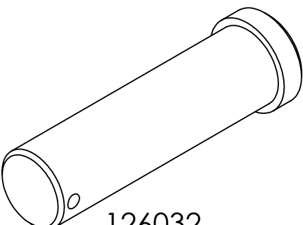
126032 Hardware: 120131 - Nut Nylock 1/4-20GR5 PLTD - QTY 1 120154 - 1" Flat Washer - QTY 1 121015 - Bolt 1/4-20 x 1-1/2 GR5 PLTD - QTY 1
