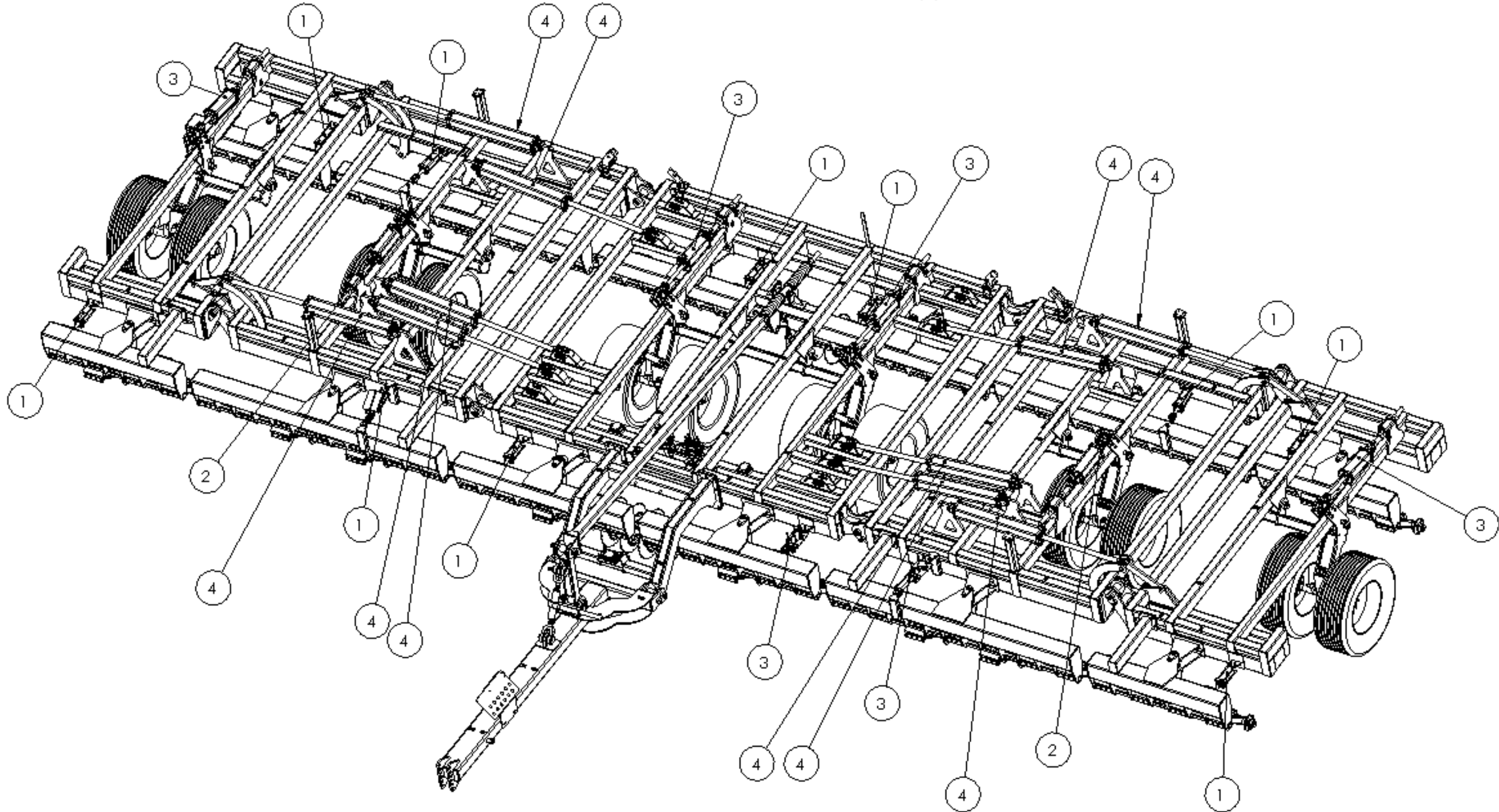
Cylinder locations on 48' and bigger units
